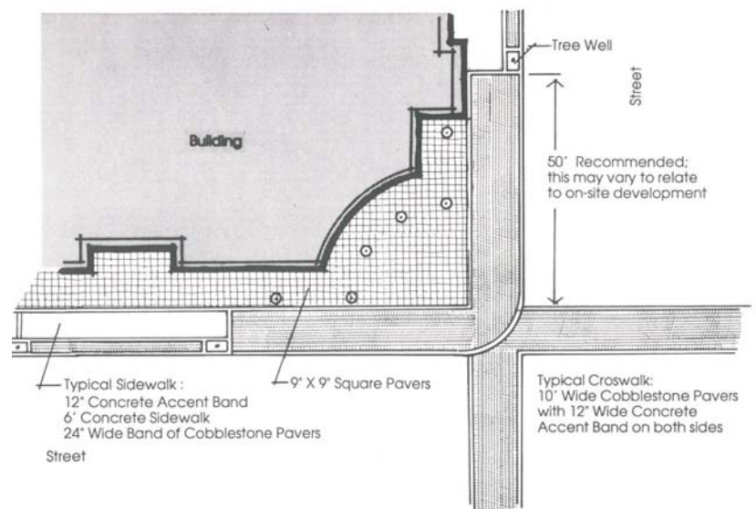
CONCEPTUAL SITE PLAN FOR PUBLIC/PRIVATE IMPROVEMENTS
